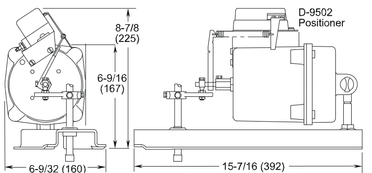
Figure 3: D-3153 Pneumatic Actuator with Universal Mounting Bracket Dimensions, in. (mm)
