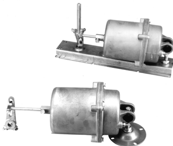
Figure 1: D-3153 Pneumatic Actuator
